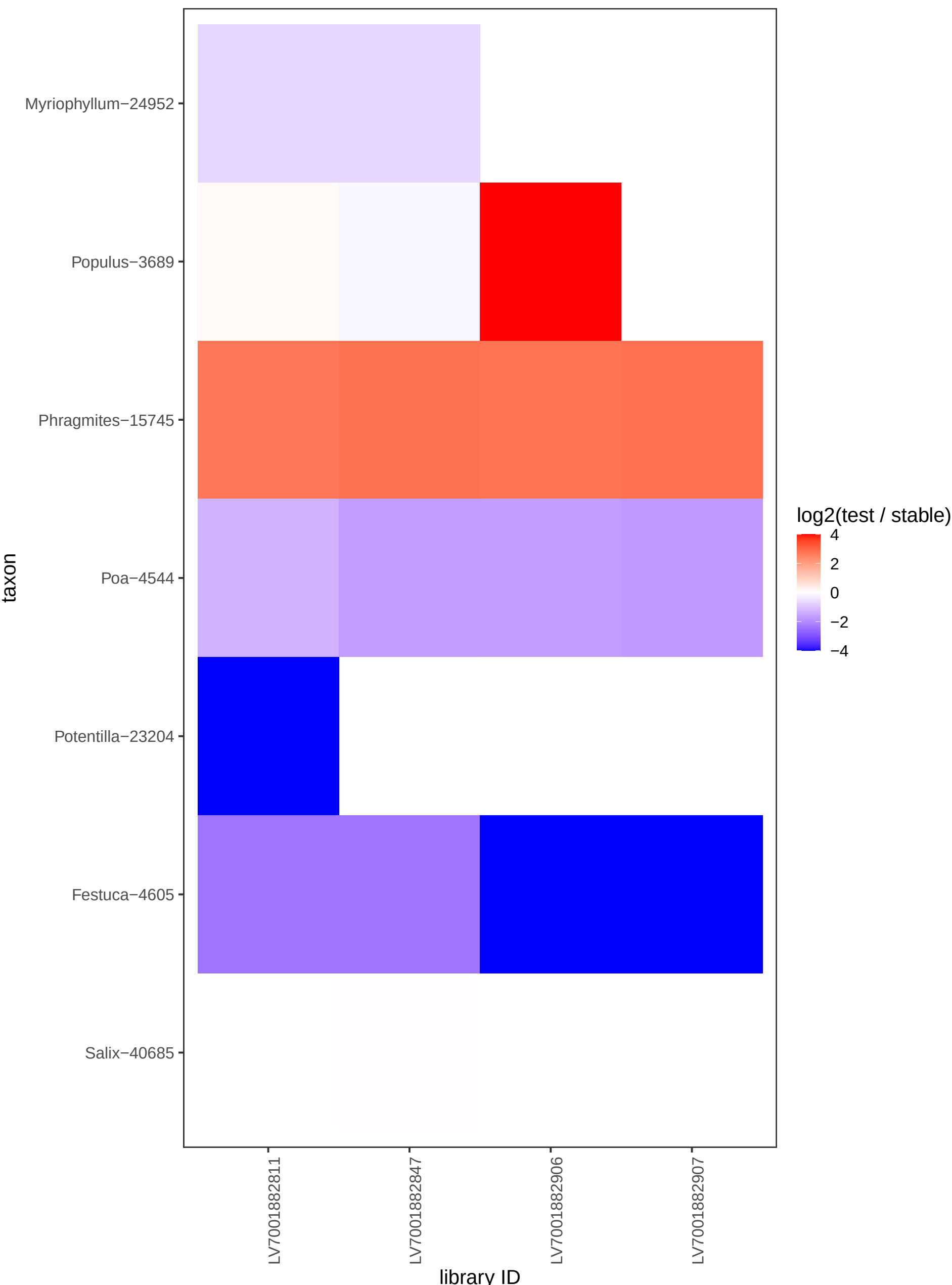
Log2 ratio heatmap (test vs stable) dataset: Hashilan marsh | Group: plant
